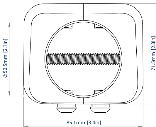
TOP VIEW - WITH COVER
