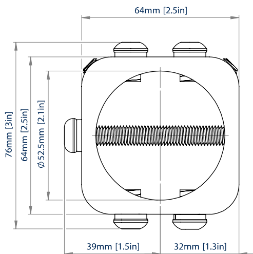
TOP VIEW - WITHOUT COVER
