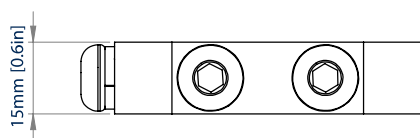
TOP VIEW - WITHOUT COVER
